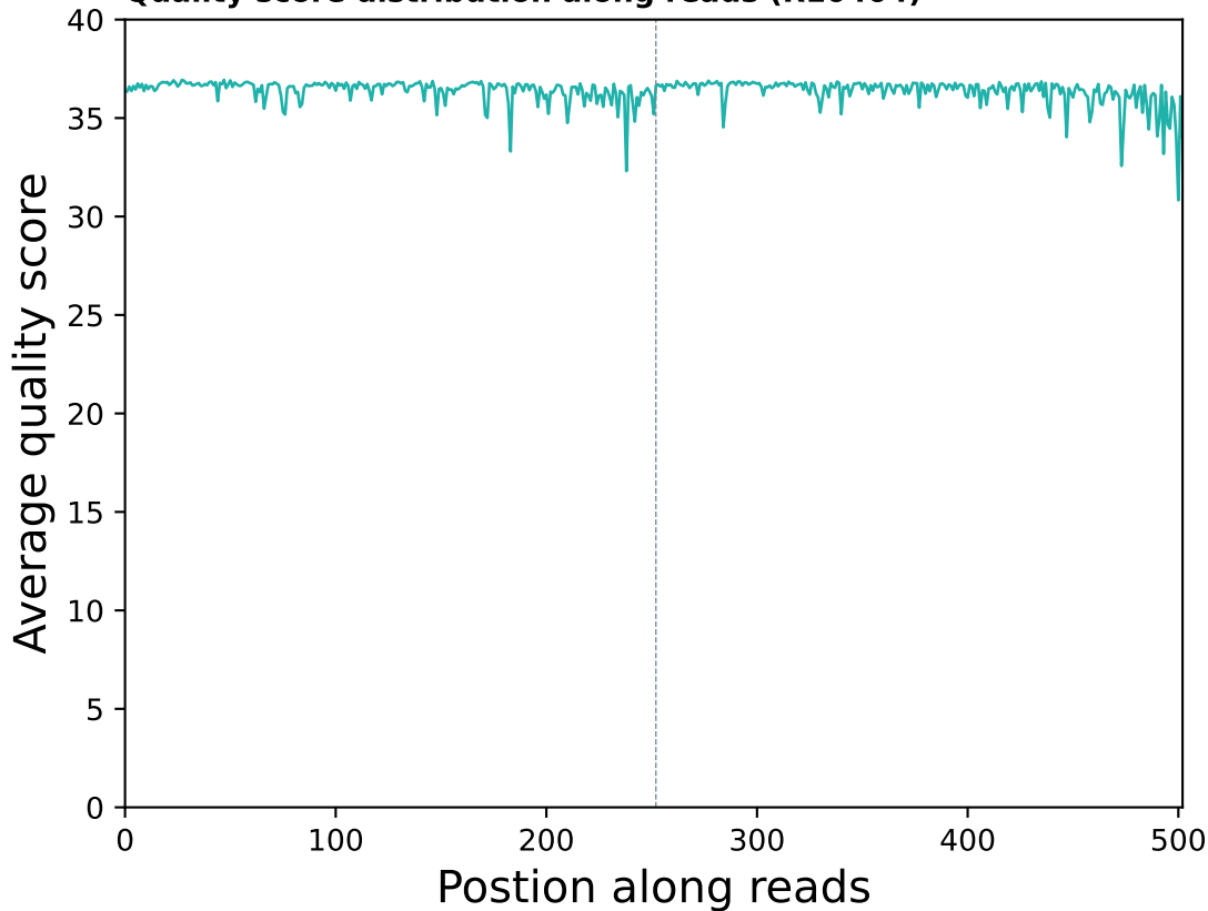
Quality score distribution along reads (R10404)
